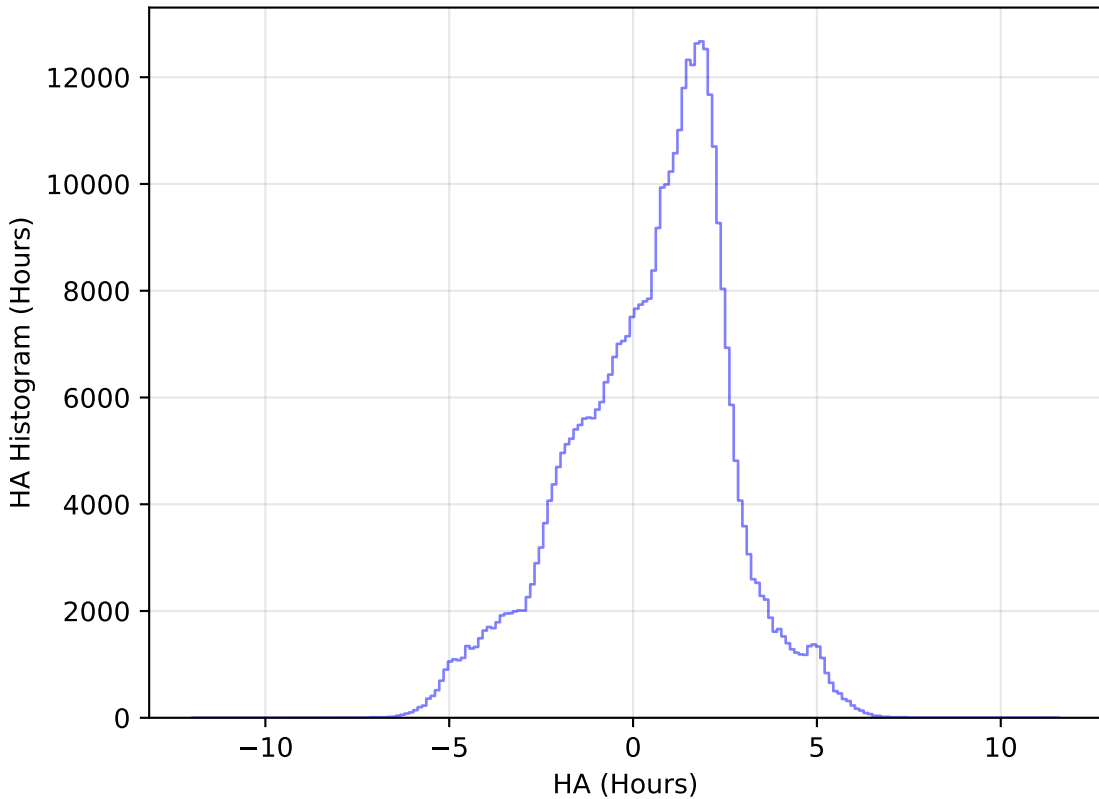
noroll_mjdp270_v3.4_10yrs WFD z band: HA Histogram
