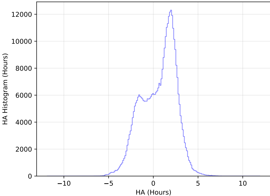
noroll_mjdp270_v3.4_10yrs WFD y band: HA Histogram
