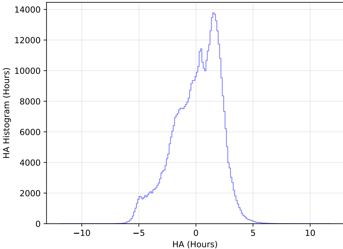
noroll_mjdp270_v3.4_10yrs WFD r band: HA Histogram
