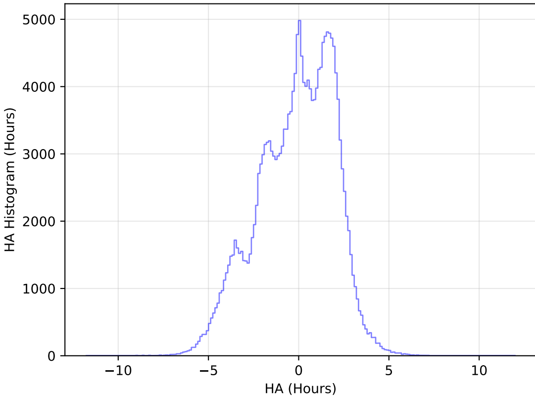
noroll_mjdp270_v3.4_10yrs WFD g band: HA Histogram
