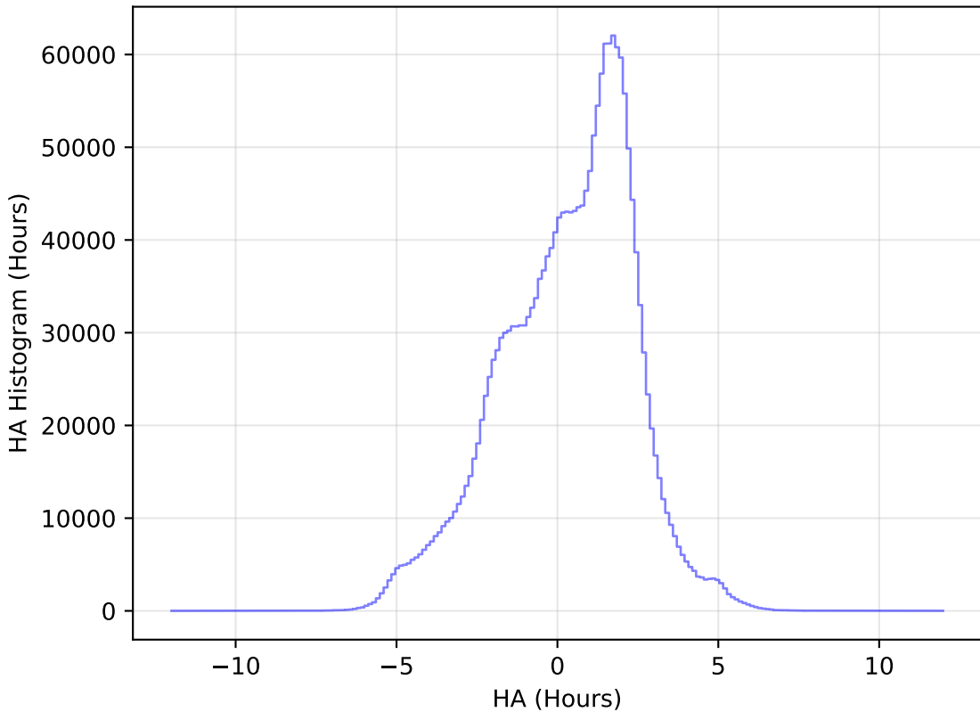
noroll_mjdp270_v3.4_10yrs WFD all bands: HA Histogram
