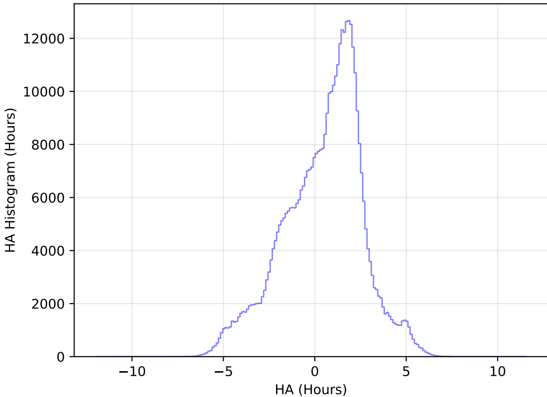
noroll_mjdp270_v3.4_10yrs All sky z band: HA Histogram
