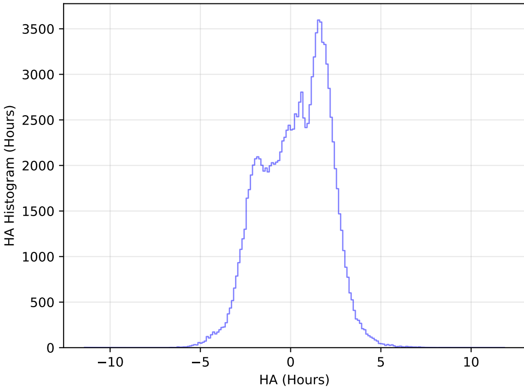
noroll_mjdp270_v3.4_10yrs All sky u band: HA Histogram
