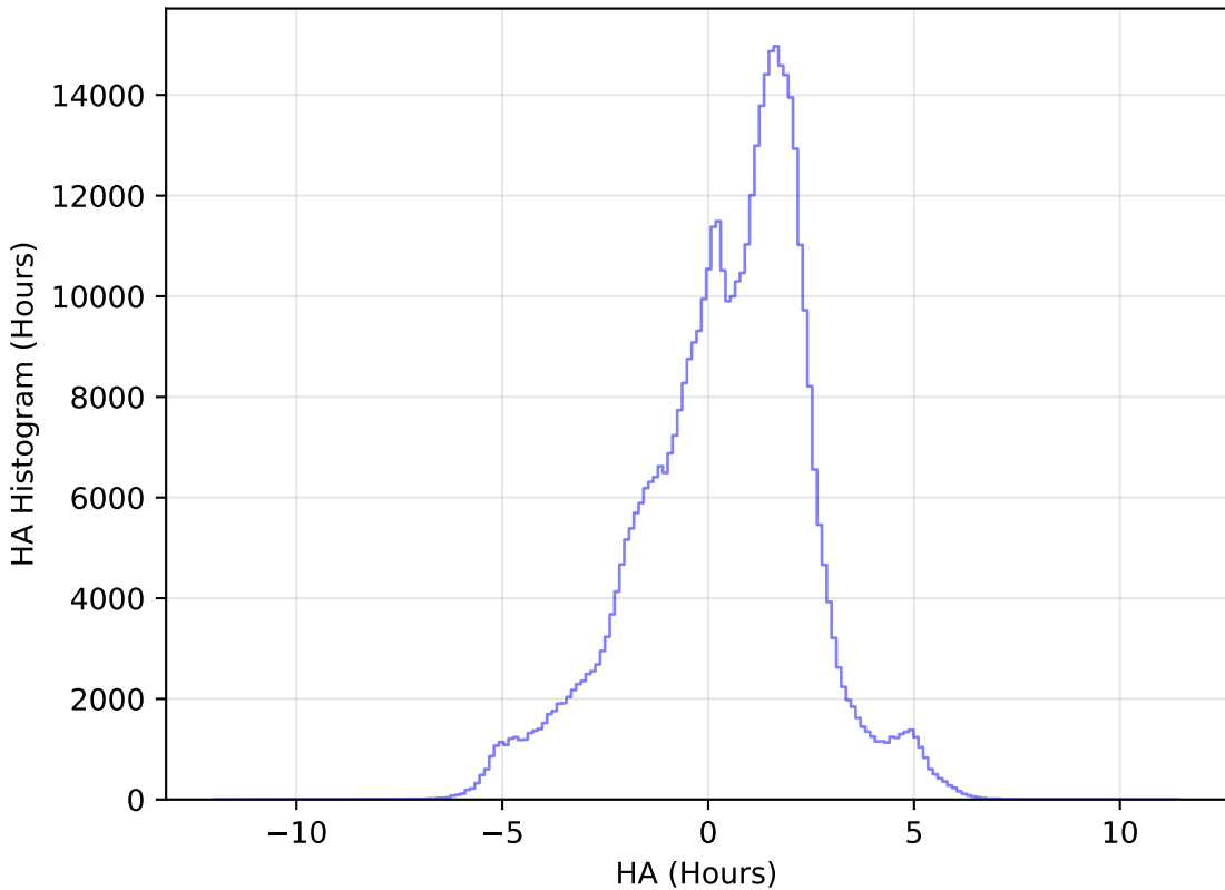
noroll_mjdp270_v3.4_10yrs All sky i band: HA Histogram
