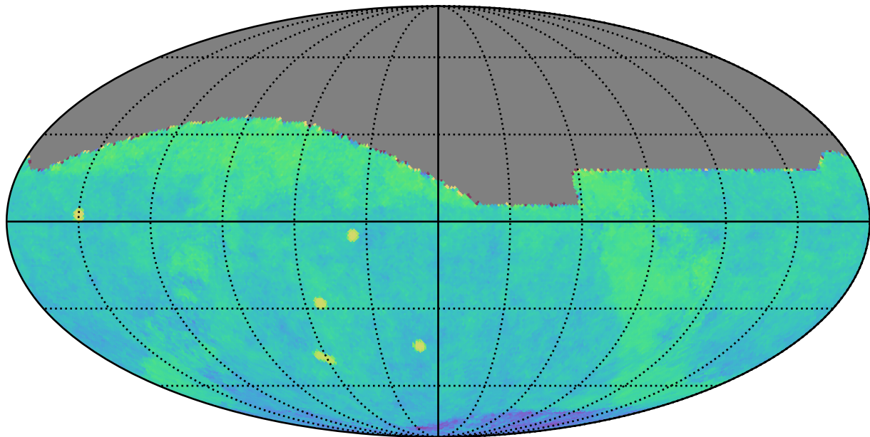
noroll_mjdp270_v3.4_10yrs gri All sky: Fraction of visits in pairs (10-60 min)
