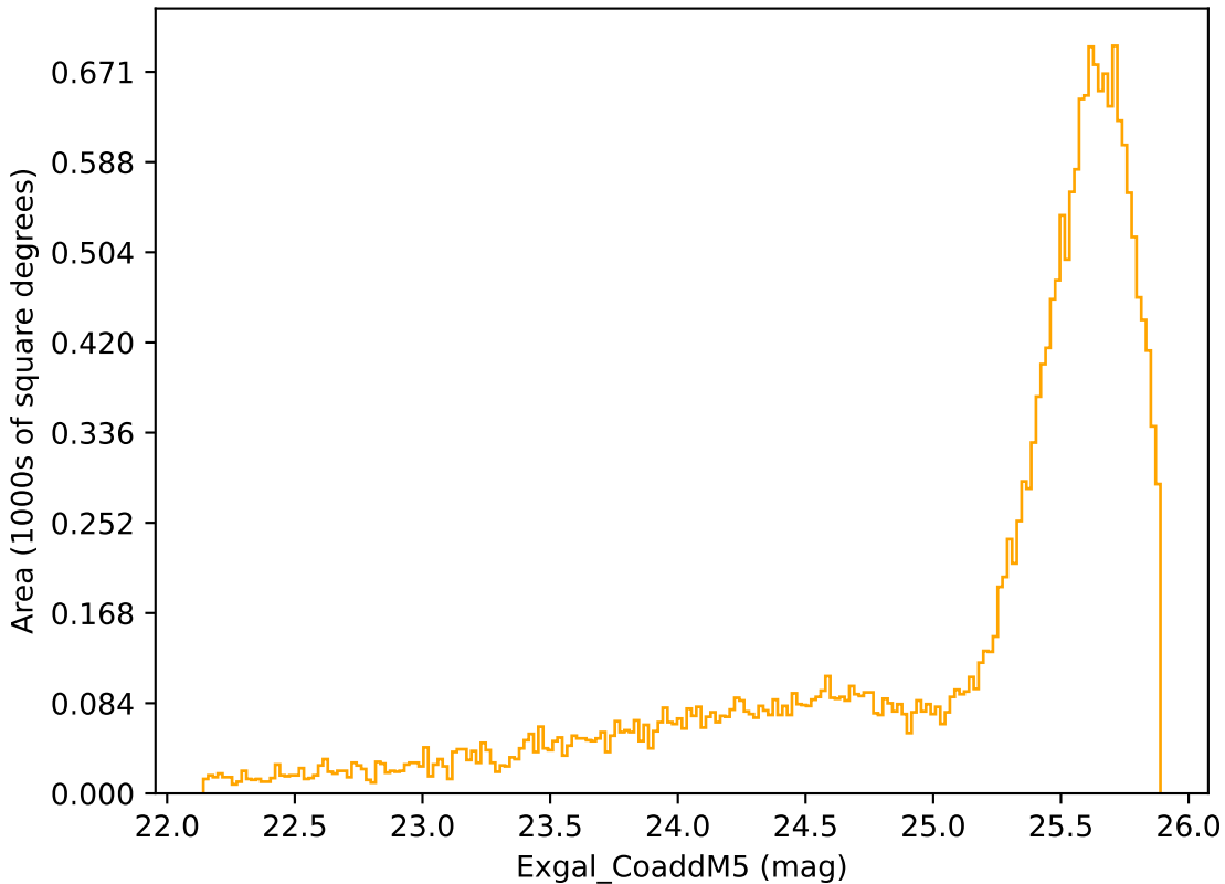
noroll_mjdp270_v3.4_10yrs Yr 3-4 r band: Exgal_CoaddM5
