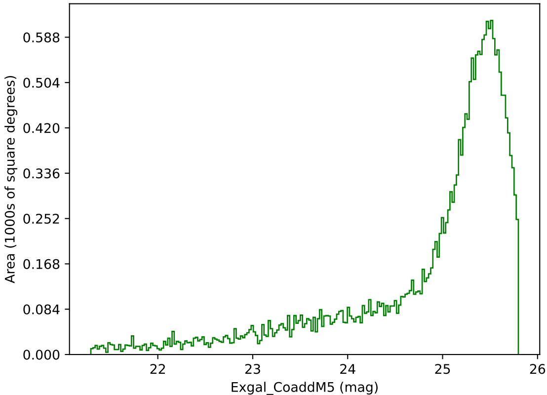
noroll_mjdp270_v3.4_10yrs Yr 3-4 g band: Exgal_CoaddM5
