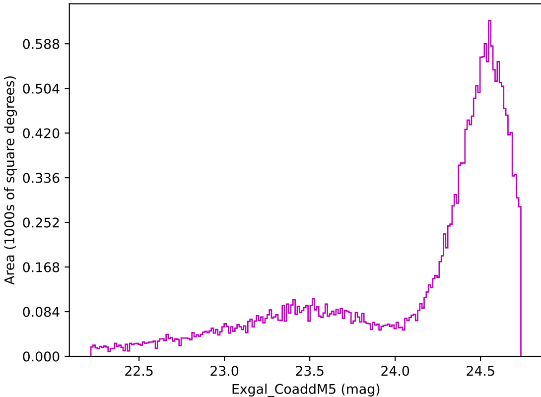
noroll_mjdp270_v3.4_10yrs Yr 1 z band: Exgal_CoaddM5
