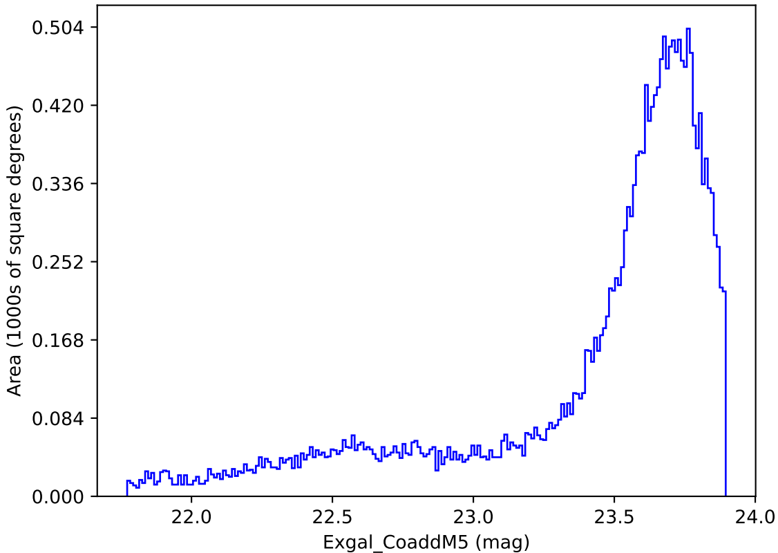
noroll_mjdp270_v3.4_10yrs Yr 1 y band: Exgal_CoaddM5
