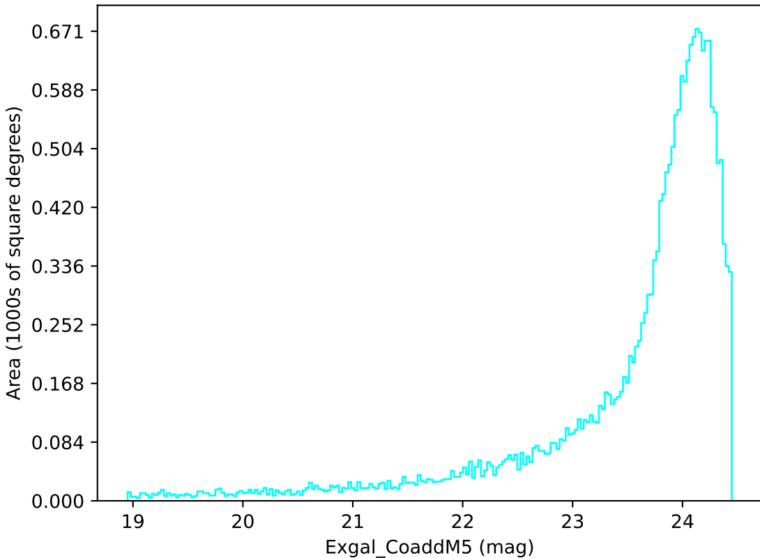
noroll_mjdp270_v3.4_10yrs Yr 1 u band: Exgal_CoaddM5
