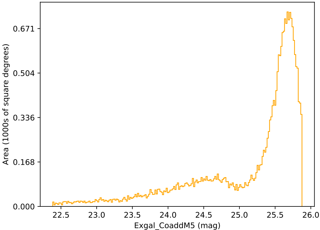
noroll_mjdp270_v3.4_10yrs Yr 1 r band: Exgal_CoaddM5
