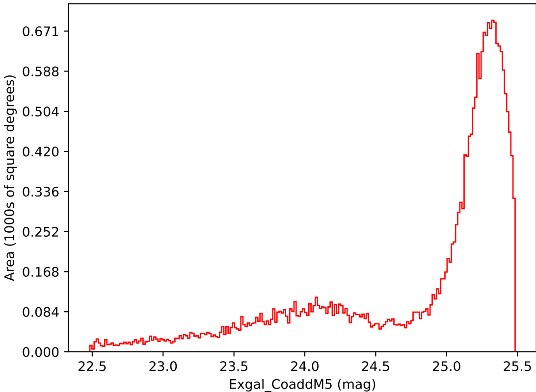
noroll_mjdp270_v3.4_10yrs Yr 1 i band: Exgal_CoaddM5
