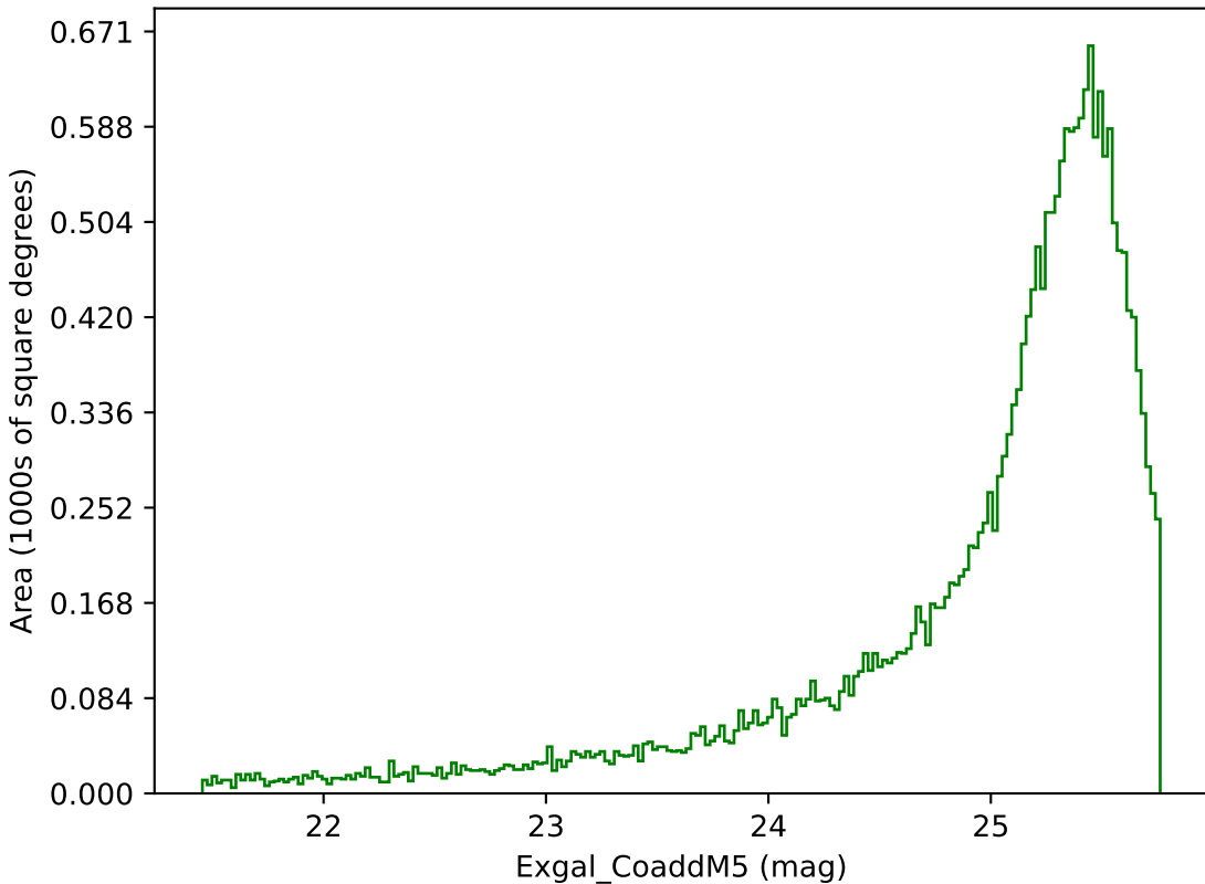
noroll_mjdp270_v3.4_10yrs Yr 1 g band: Exgal_CoaddM5
