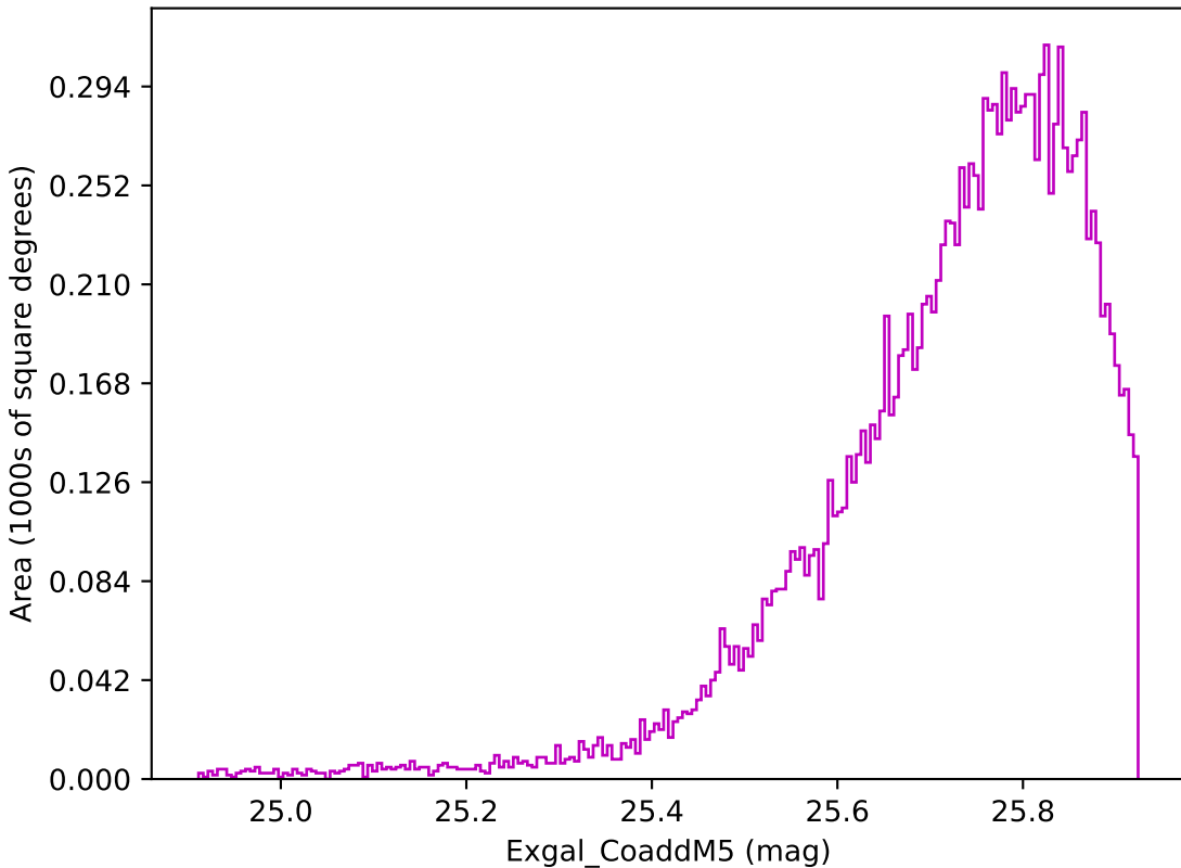
noroll_mjdp270_v3.4_10yrs WFD z band: Exgal_CoaddM5
