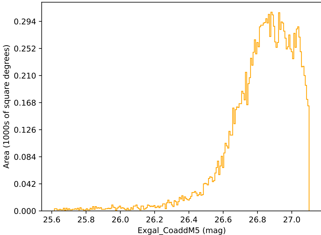
noroll_mjdp270_v3.4_10yrs WFD r band: Exgal_CoaddM5
