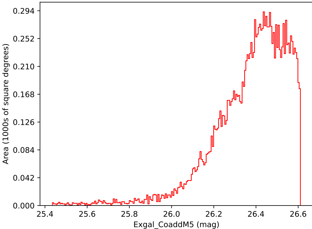
noroll_mjdp270_v3.4_10yrs WFD i band: Exgal_CoaddM5
