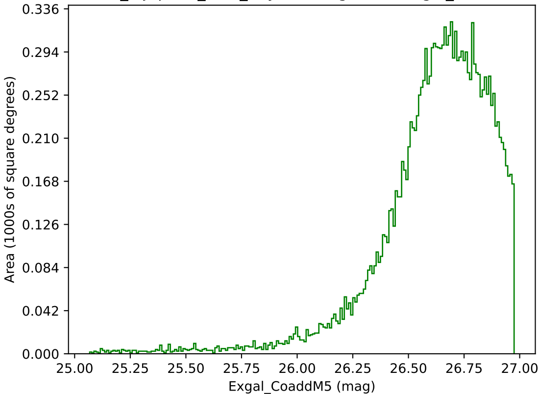
noroll_mjdp270_v3.4_10yrs WFD g band: Exgal_CoaddM5
