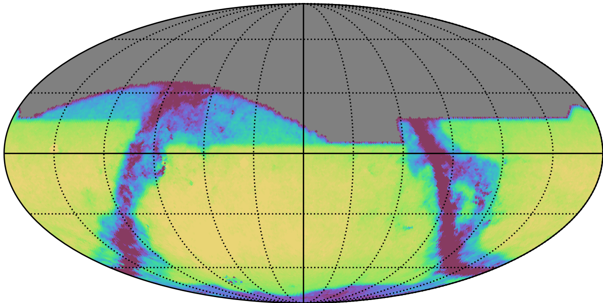
noroll_mjdp270_v3.4_10yrs All sky z band: Exgal_CoaddM5
