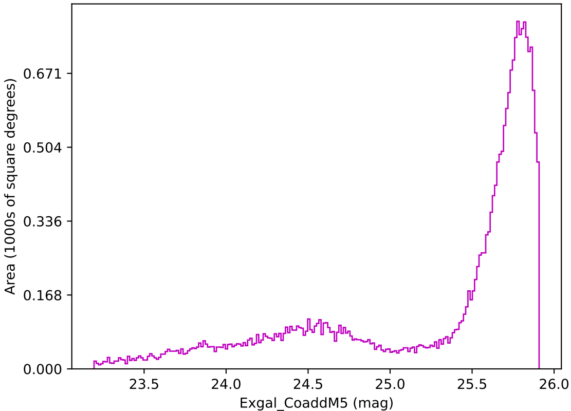
noroll_mjdp270_v3.4_10yrs All sky z band: Exgal_CoaddM5
