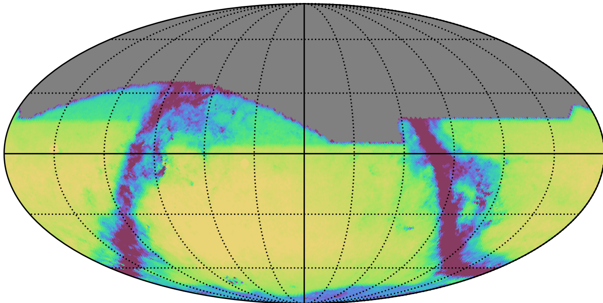
noroll_mjdp270_v3.4_10yrs All sky r band: Exgal_CoaddM5
