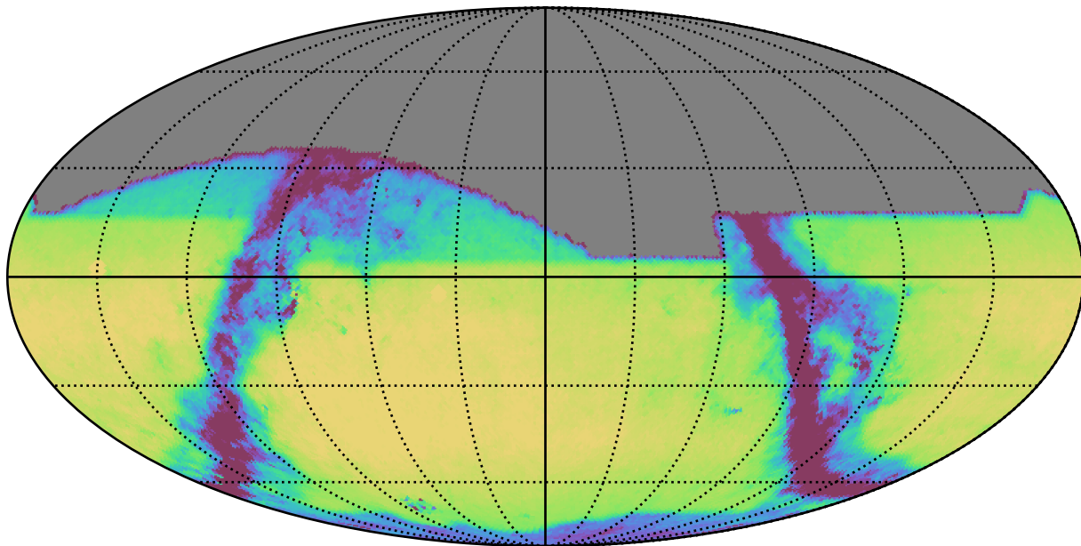
noroll_mjdp270_v3.4_10yrs All sky i band: Exgal_CoaddM5
