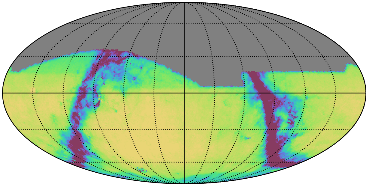
noroll_mjdp270_v3.4_10yrs All sky g band: Exgal_CoaddM5
