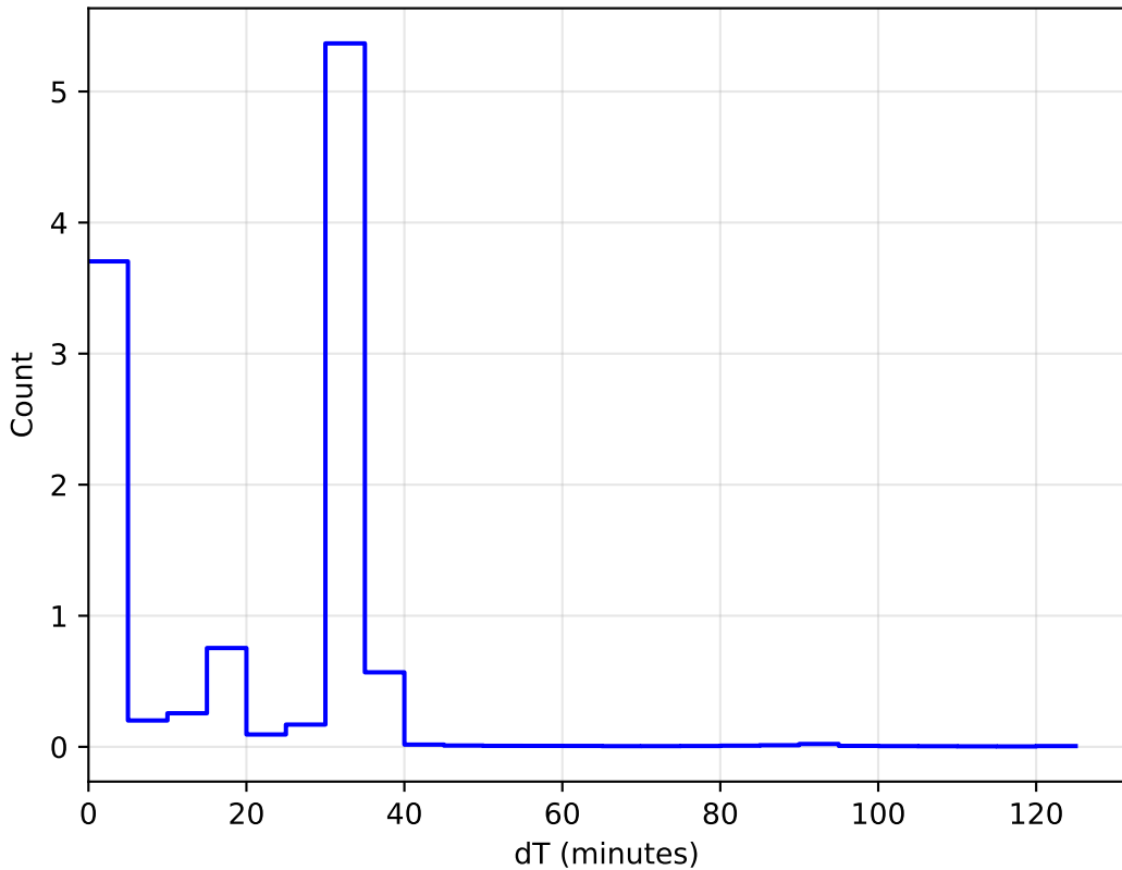
1e6 noroll_mjdp270_v3.4_10yrs WFD: DeltaT Histogram
