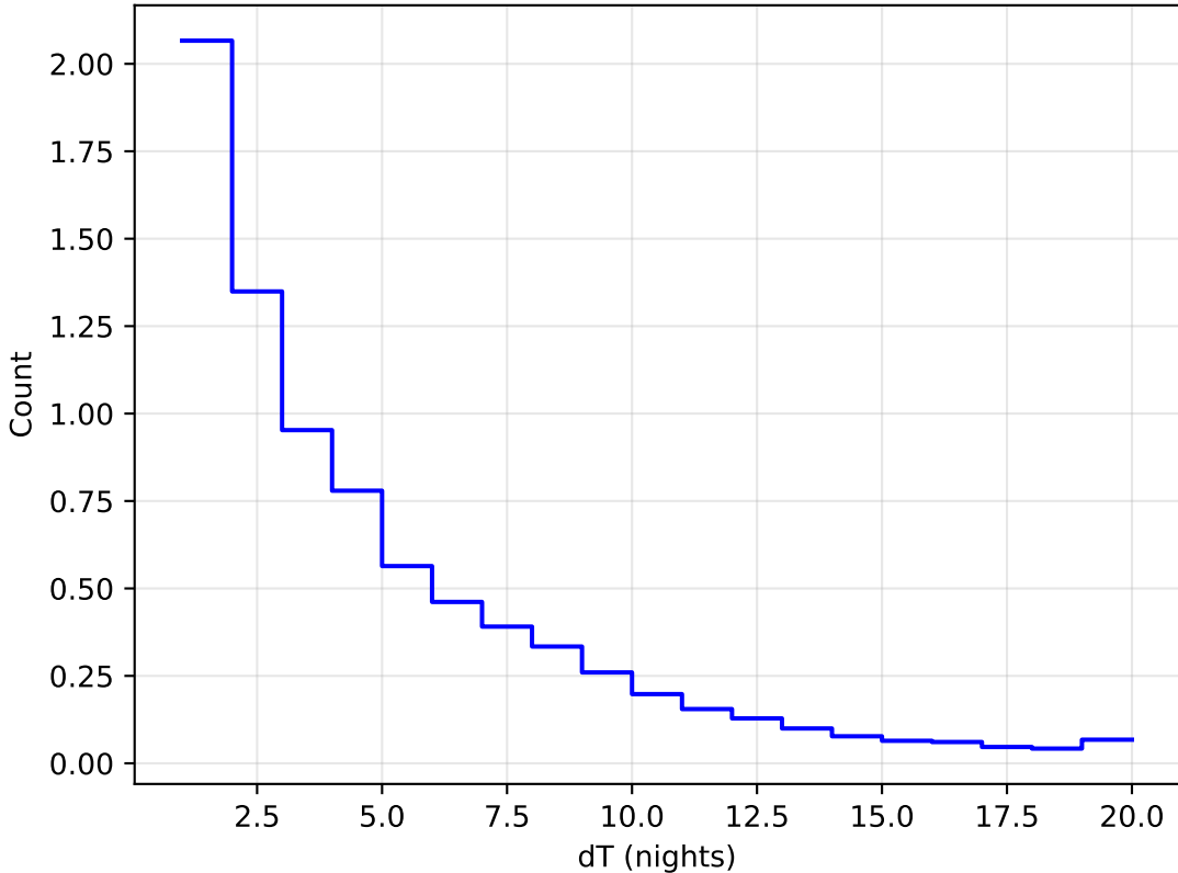
noroll_mjdp270_v3.4_10yrs WFD all bands: DeltaNight Histogram
