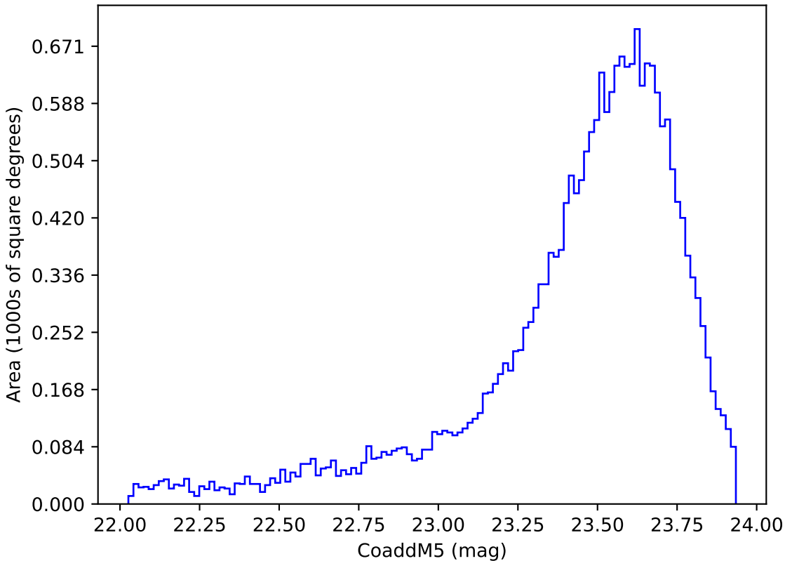
noroll_mjdp270_v3.4_10yrs Yr 3-4 y band: CoaddM5
