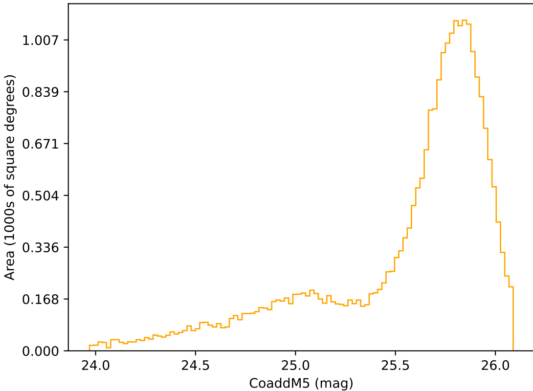
noroll_mjdp270_v3.4_10yrs Yr 3-4 r band: CoaddM5
