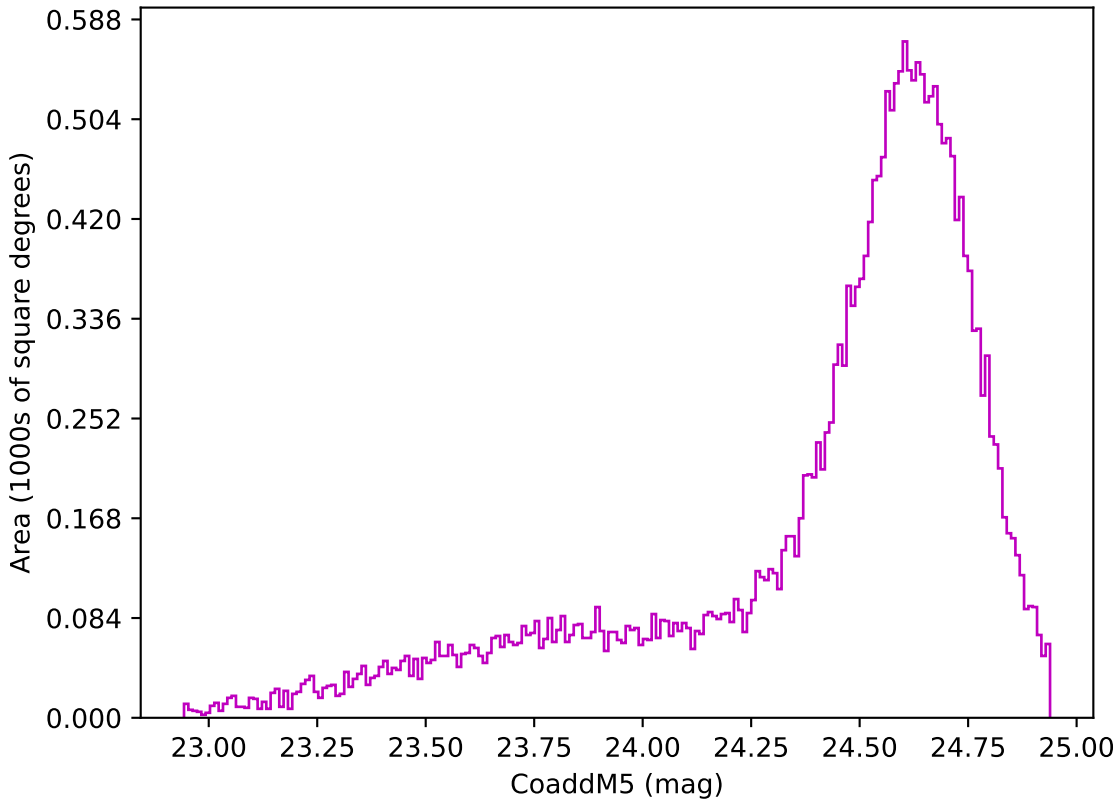
noroll_mjdp270_v3.4_10yrs Yr 1 z band: CoaddM5
