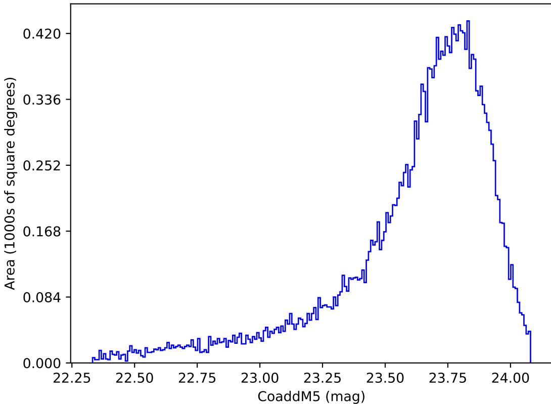
noroll_mjdp270_v3.4_10yrs Yr 1 y band: CoaddM5
