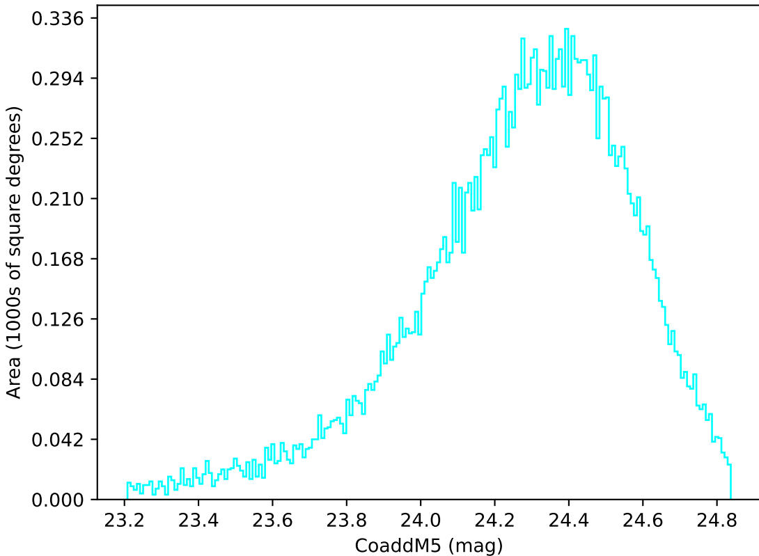
noroll_mjdp270_v3.4_10yrs Yr 1 u band: CoaddM5
