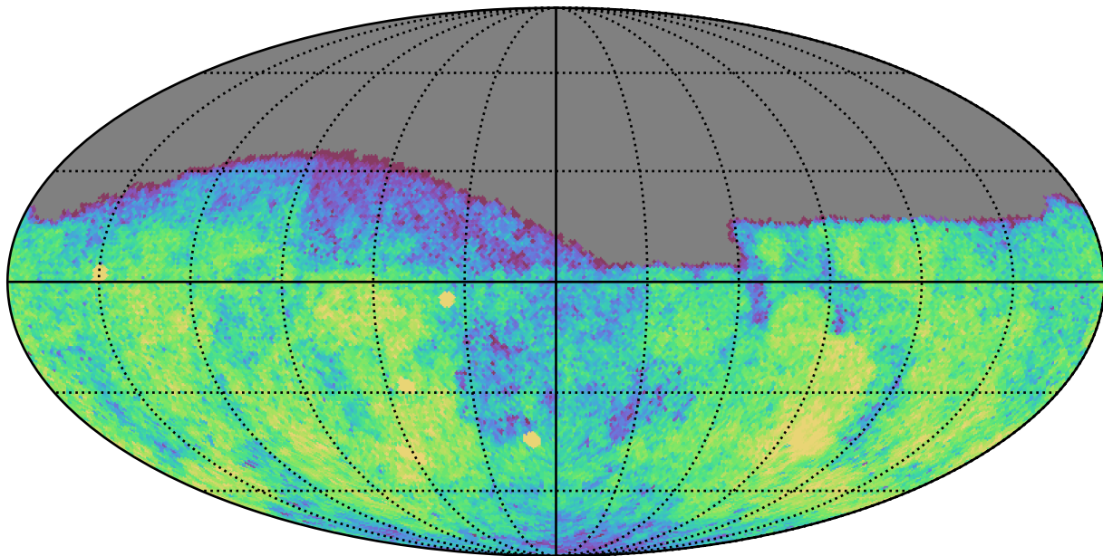
noroll_mjdp270_v3.4_10yrs Yr 1 g band: CoaddM5
