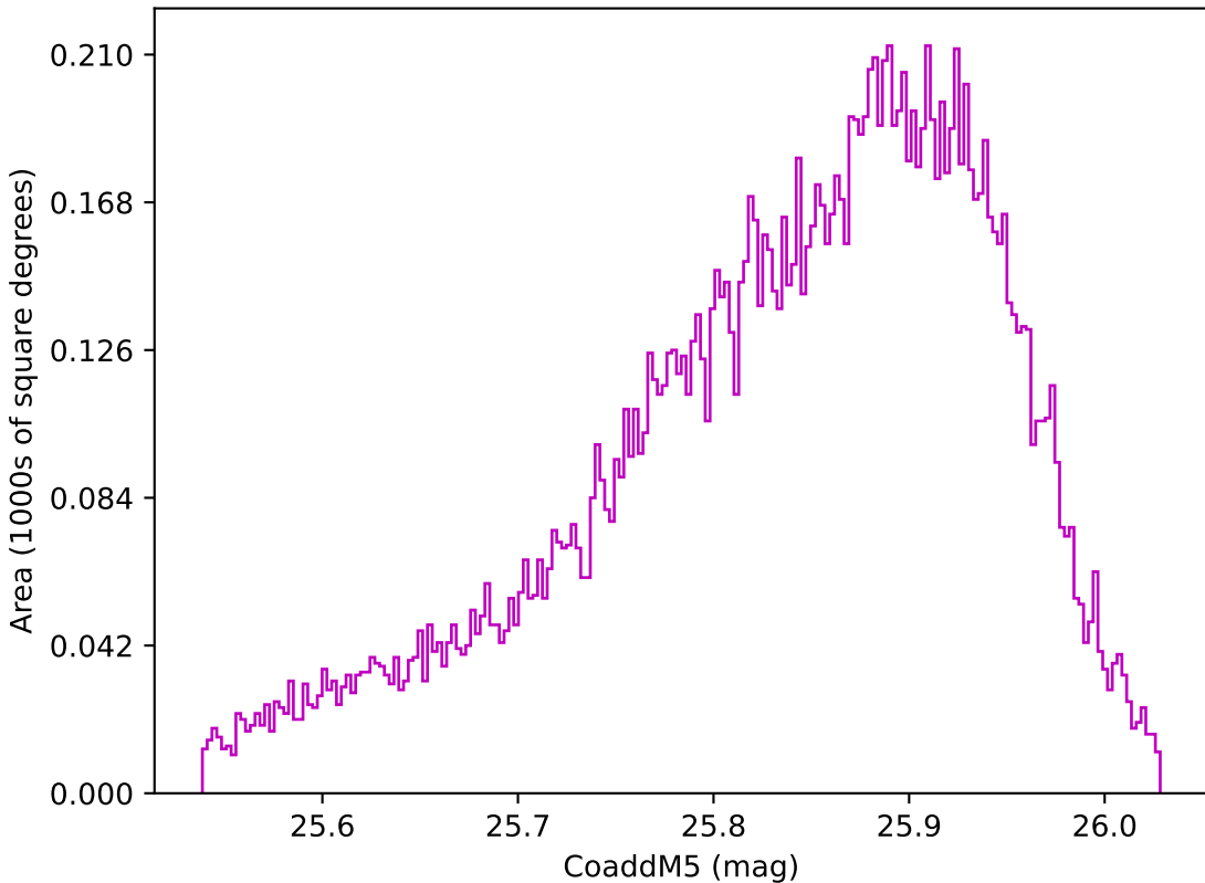
noroll_mjdp270_v3.4_10yrs WFD z band: CoaddM5
