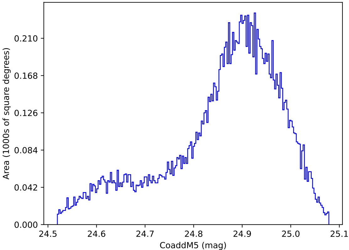
noroll_mjdp270_v3.4_10yrs WFD y band: CoaddM5
