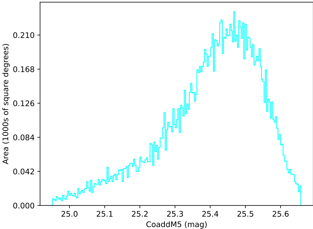
noroll_mjdp270_v3.4_10yrs WFD u band: CoaddM5
