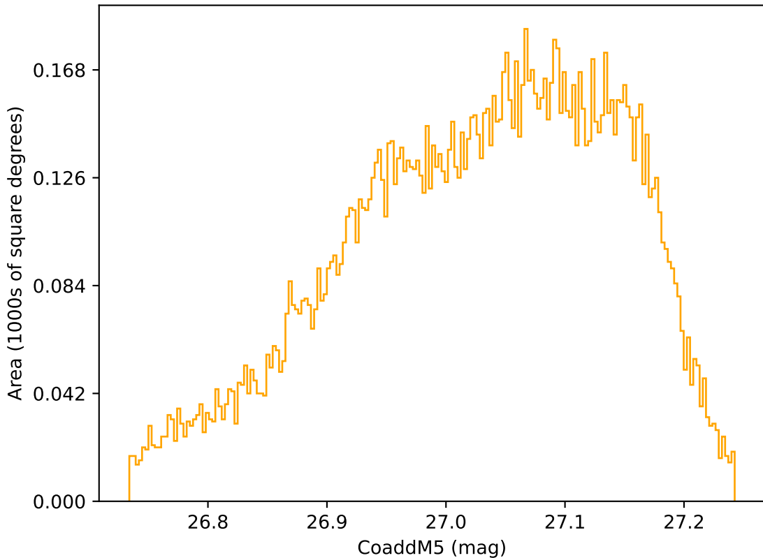
noroll_mjdp270_v3.4_10yrs WFD r band: CoaddM5
