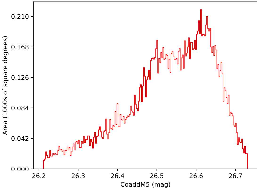
noroll_mjdp270_v3.4_10yrs WFD i band: CoaddM5
