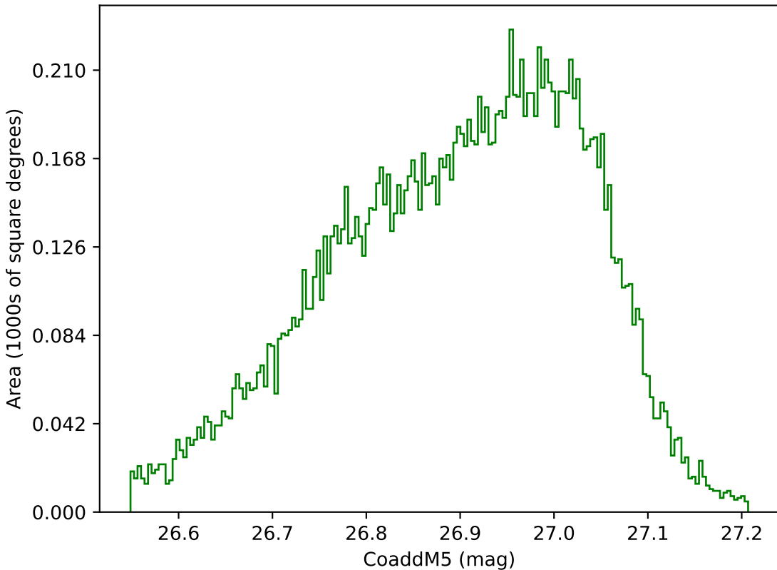
noroll_mjdp270_v3.4_10yrs WFD g band: CoaddM5
