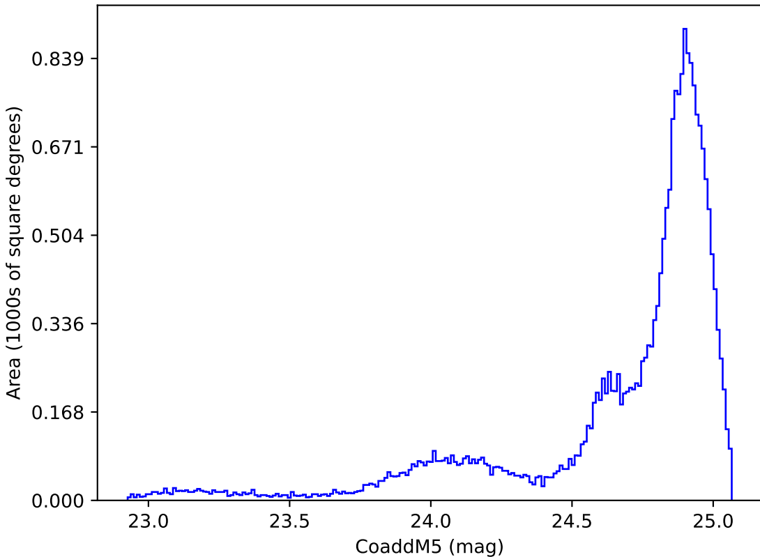
noroll_mjdp270_v3.4_10yrs All sky y band: CoaddM5
