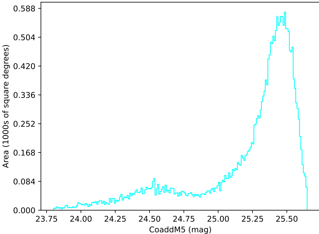
noroll_mjdp270_v3.4_10yrs All sky u band: CoaddM5
