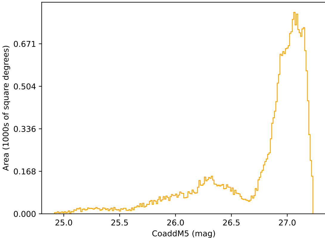
noroll_mjdp270_v3.4_10yrs All sky r band: CoaddM5
