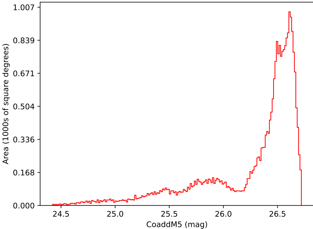
noroll_mjdp270_v3.4_10yrs All sky i band: CoaddM5
