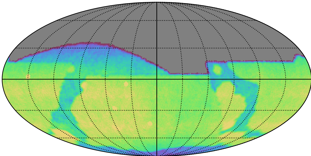
noroll_mjdp270_v3.4_10yrs All sky g band: CoaddM5
