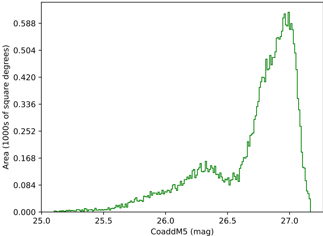
noroll_mjdp270_v3.4_10yrs All sky g band: CoaddM5
