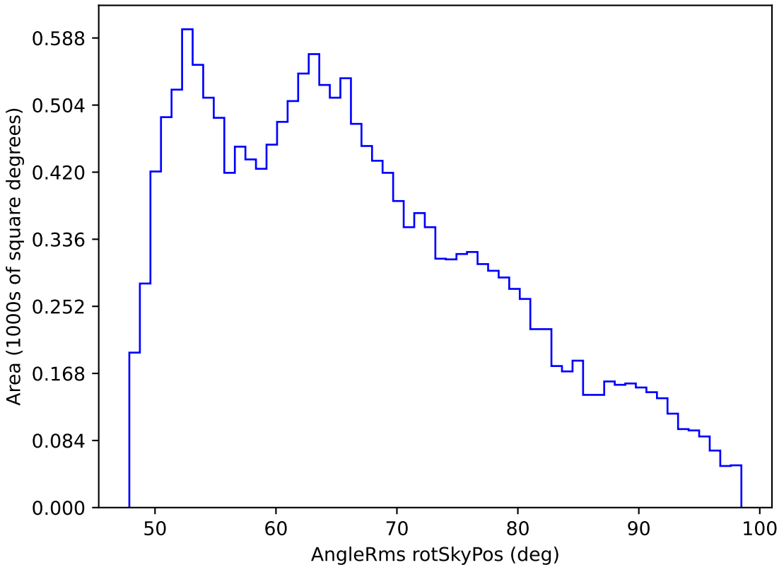
noroll_mjdp270_v3.4_10yrs WFD z band: AngleRms rotSkyPos
