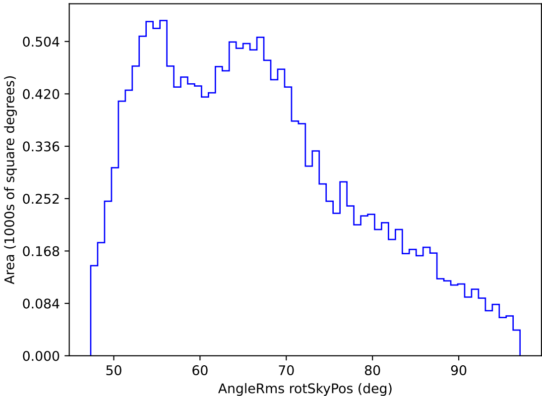
noroll_mjdp270_v3.4_10yrs WFD y band: AngleRms rotSkyPos
