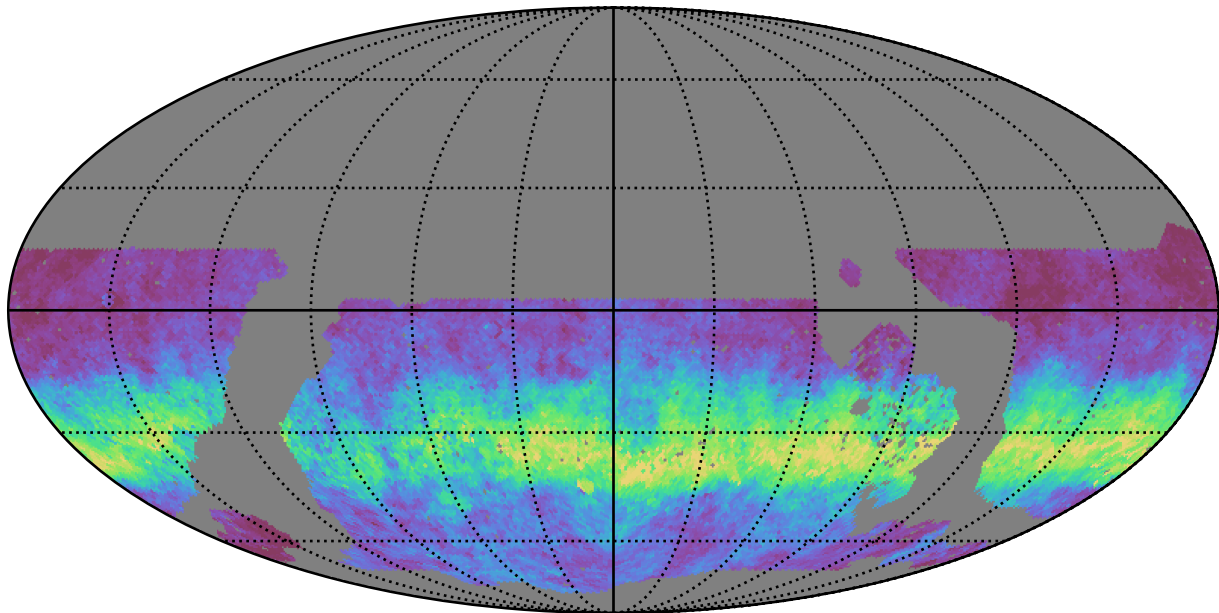
noroll_mjdp270_v3.4_10yrs WFD u band: AngleRms rotSkyPos
