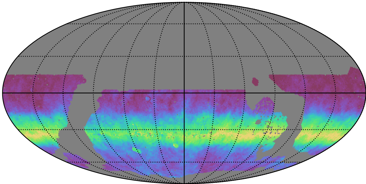
noroll_mjdp270_v3.4_10yrs WFD r band: AngleRms rotSkyPos
